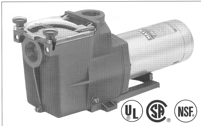
SP2610X15 1 1/2 H.P. Super Pump.
