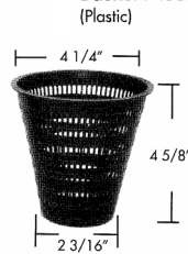
B - 211 Muskin Pump Basket 097-6902 (Plastic)
